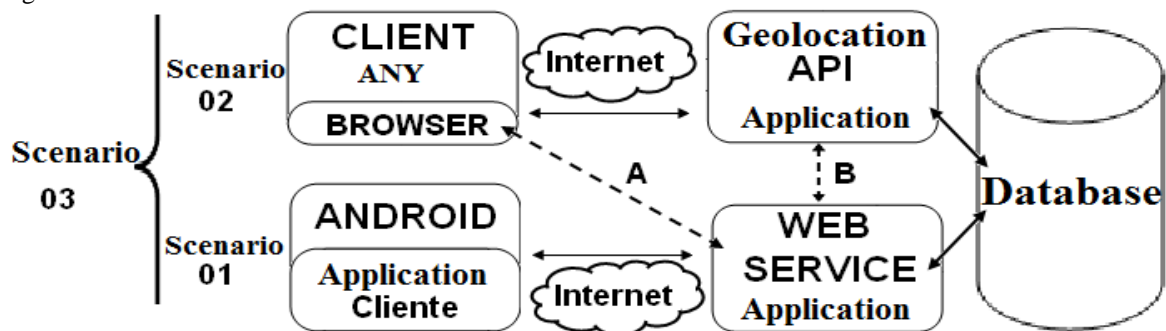
Figure 4. Implementation Scenarios of the SocialNetLab
